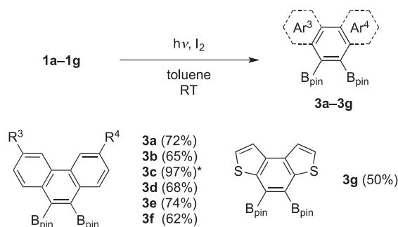
Scheme 3. Preparation of 1,2-diborylarenes 3 (in the case of 3c , the reaction was carried out in the presence of propylene oxide).
