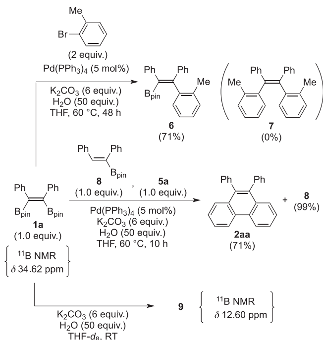
Scheme 4. Experiments performed using 1a for elucidation of the mechanism.
