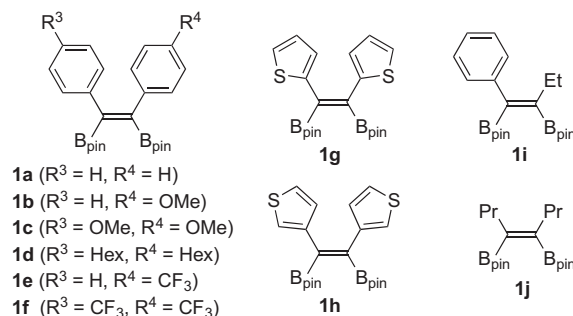
Fig. 1. Molecular structures of 1 .
