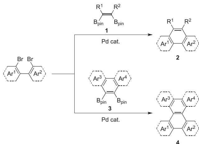
Scheme 2. Palladium-catalyzed annulation of 1,2-diboryl reagents 1 and 3 with 2,2'-dibromobiaryls (B pin : pinacolatoboryl).
