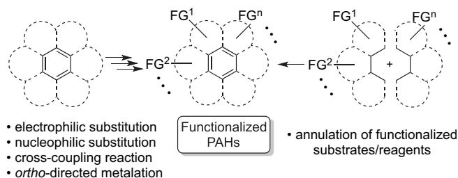
Scheme 1. Synthetic approach to functionalized PAHs (FG: functional group).
